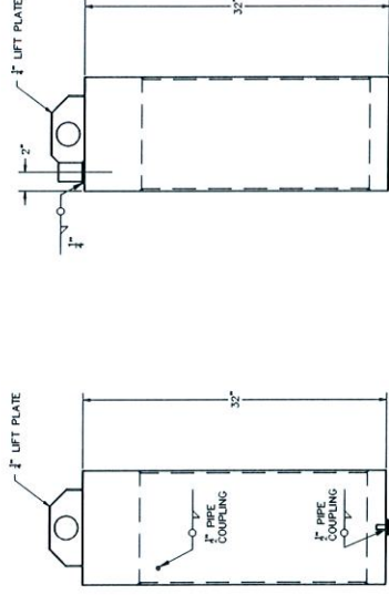
DRIVER SIDE VIEW
