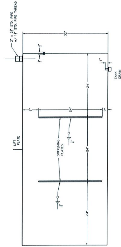
CUTAWAY FRONT VIEW
